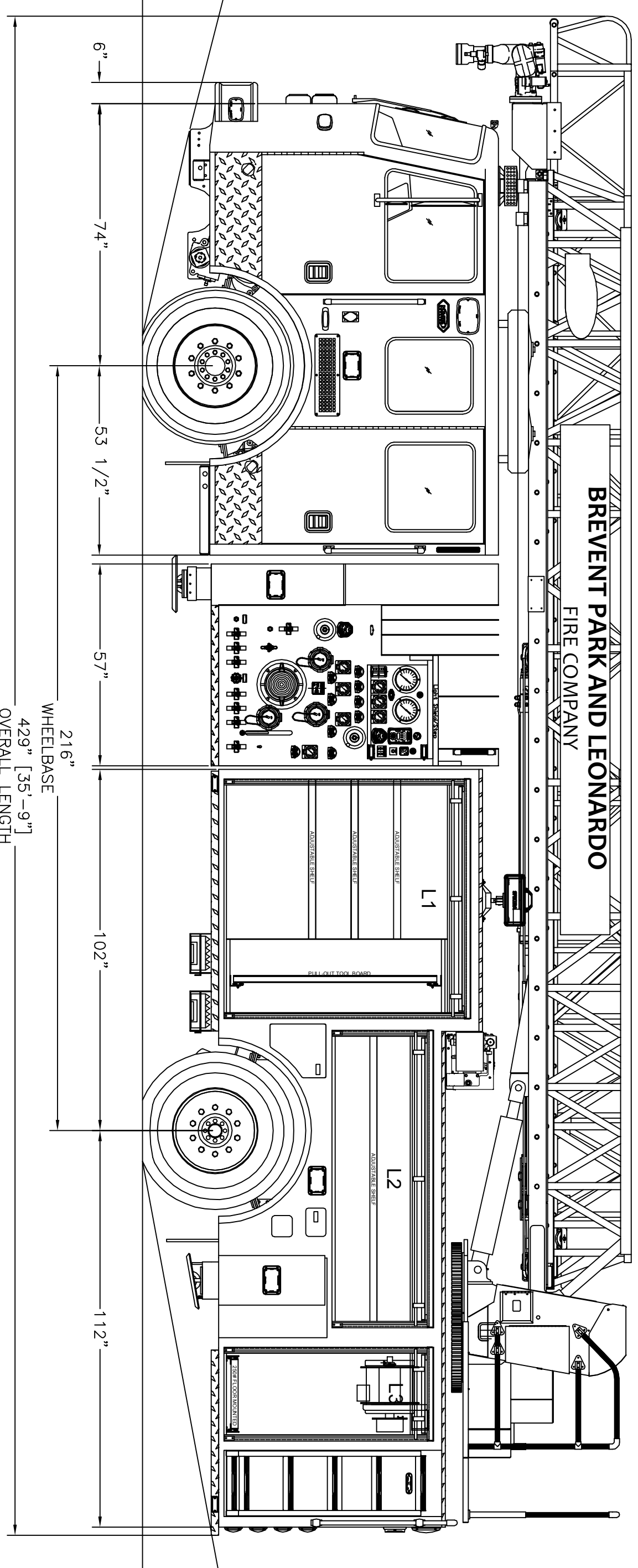
DRIVERS SIDE VIEW
